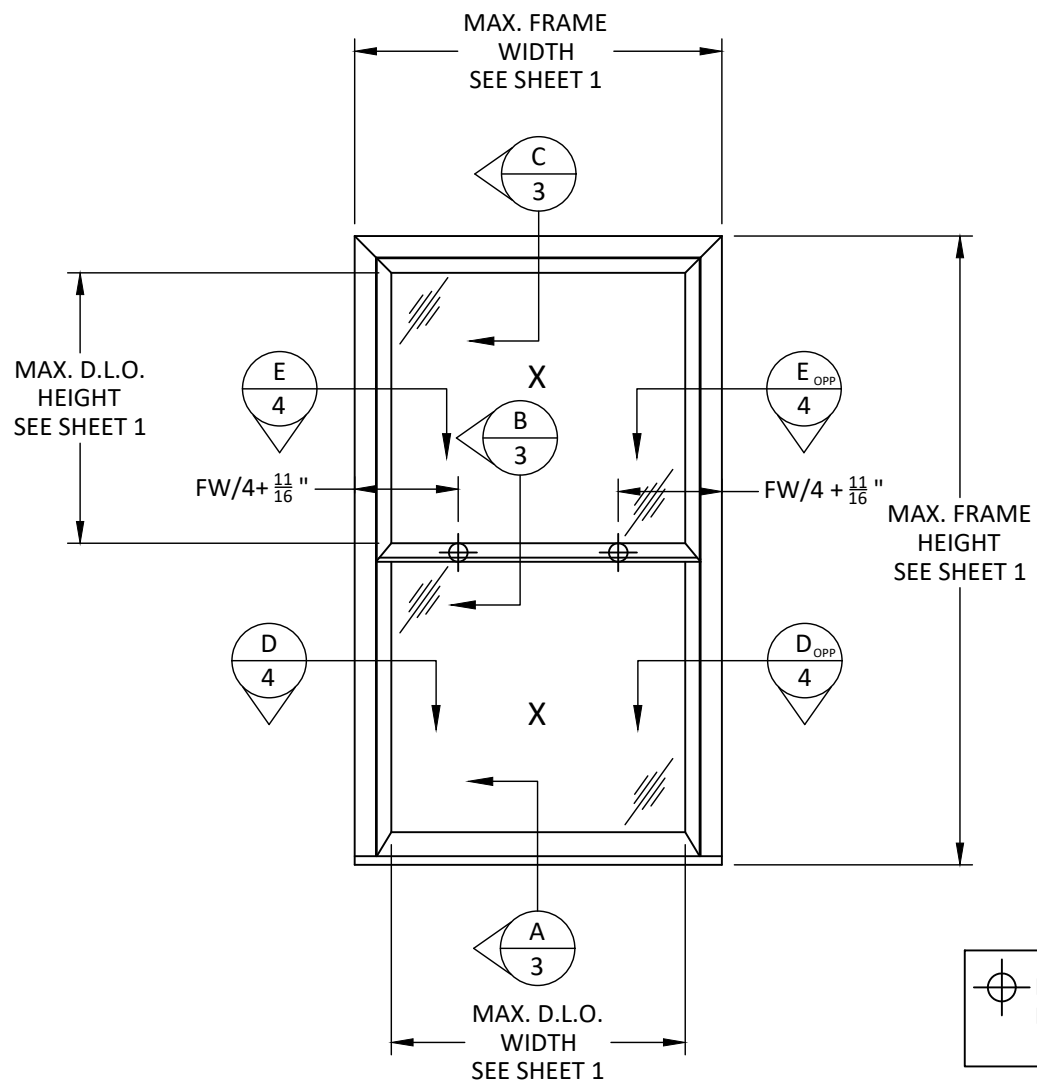
ELEVATION TYPICAL
